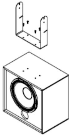
Figure 2-3 Installing the Yoke on the CSB115/CSB115-CM
