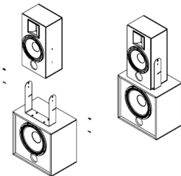
Figure 2-4 Attaching the CS50-CM or CS50-CM to the CSB115/CSB115-CM
