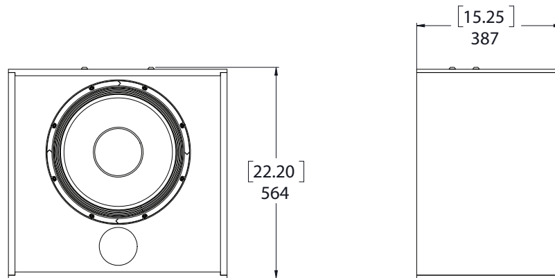
Figure 2-5 CSB115 and CSB115-CM [Inches] and Millimeters
