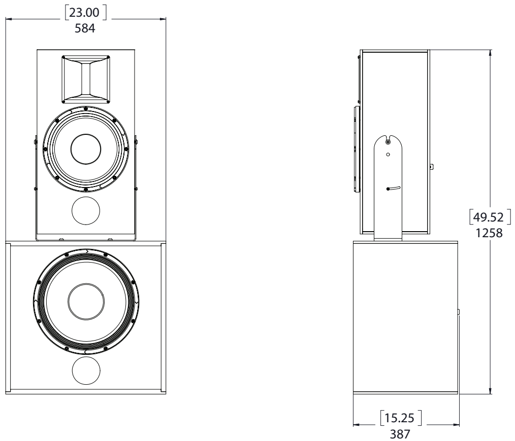
Figure 2-6 CSB115/CSB115-CM with CS50-CM (System 100A) [Inches] and Millimeters
